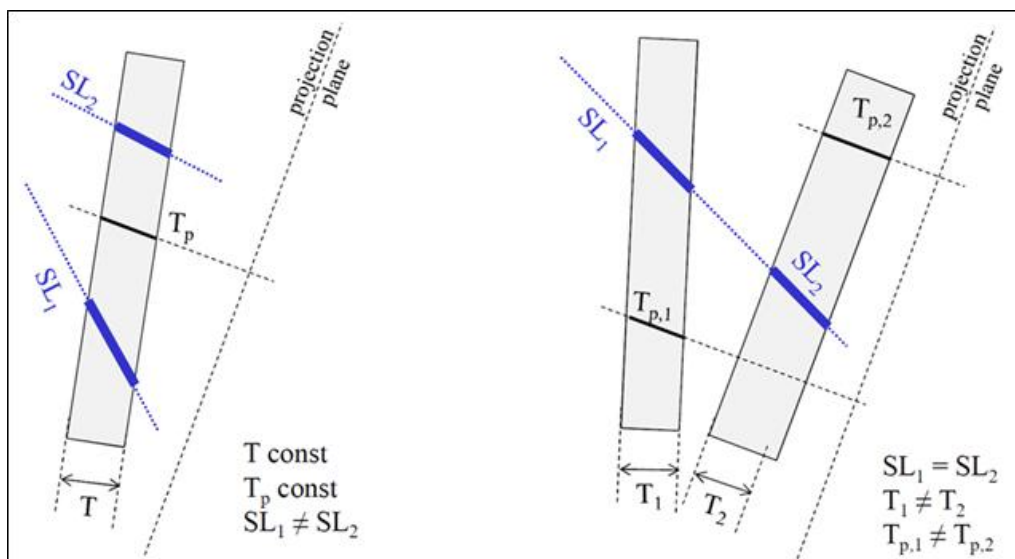
Figure 11-4: Geometric relationship between drillhole intersection and length, and true and projected thickness
