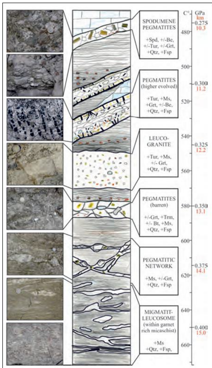
Figure 6-4: Proposed genetic model for the formation of Alpine Permian pegmatites
