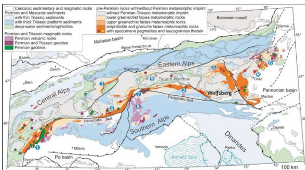
Figure 6-1: Geological map of the Alps showing the distribution of Permian metamorphism and related magmatic rocks (including spodumene-bearing pegmatites)
