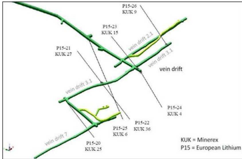
Figure 9-3: 3D view illustrating Minerex drillholes selected for the twin hole verification program in 2016 (drillhole spacing approximately 100 m)
