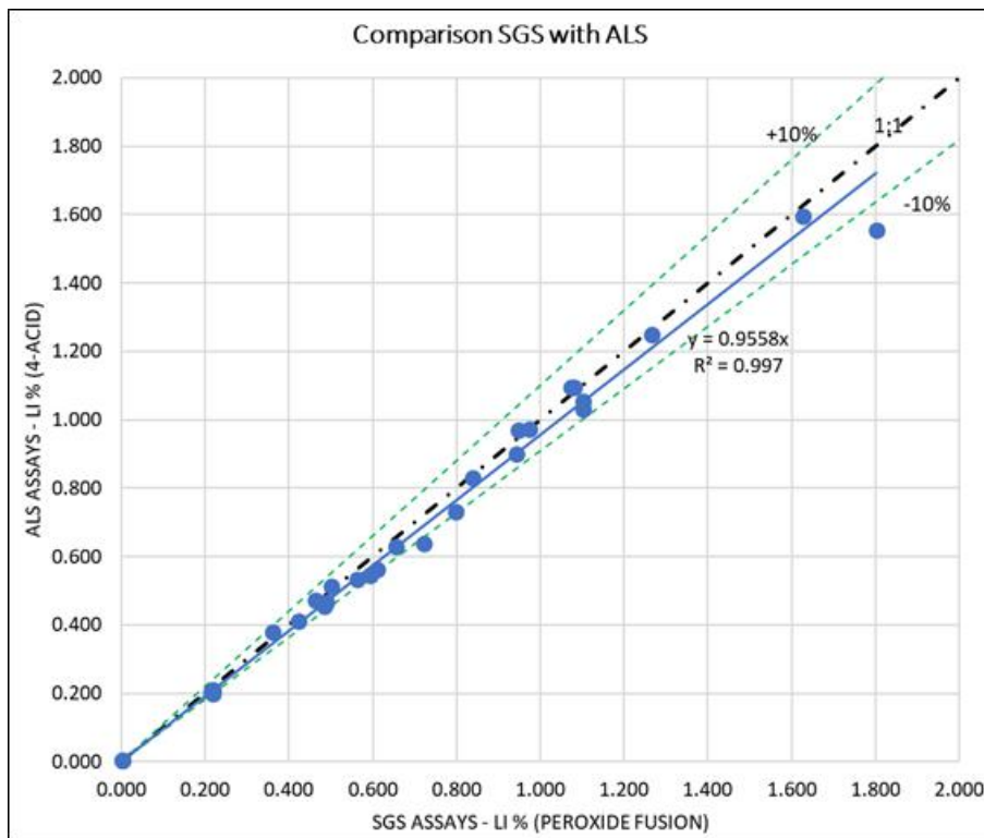
Figure 8-5: Results of check lab analysis results from SGS of 29 sample from 2016 exploration program
