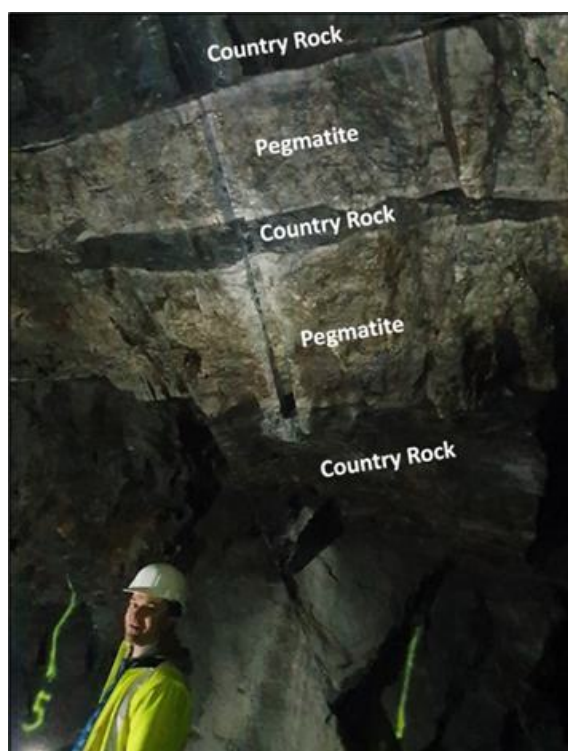
Figure 9-9: Pegmatite exposure in the roof of an exploration drift; note the internal country rock and channel sample
