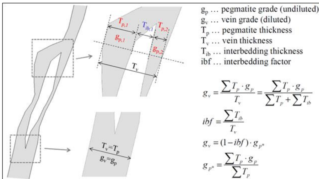
Figure 11-5: Thickness and grade of the pegmatite and vein
