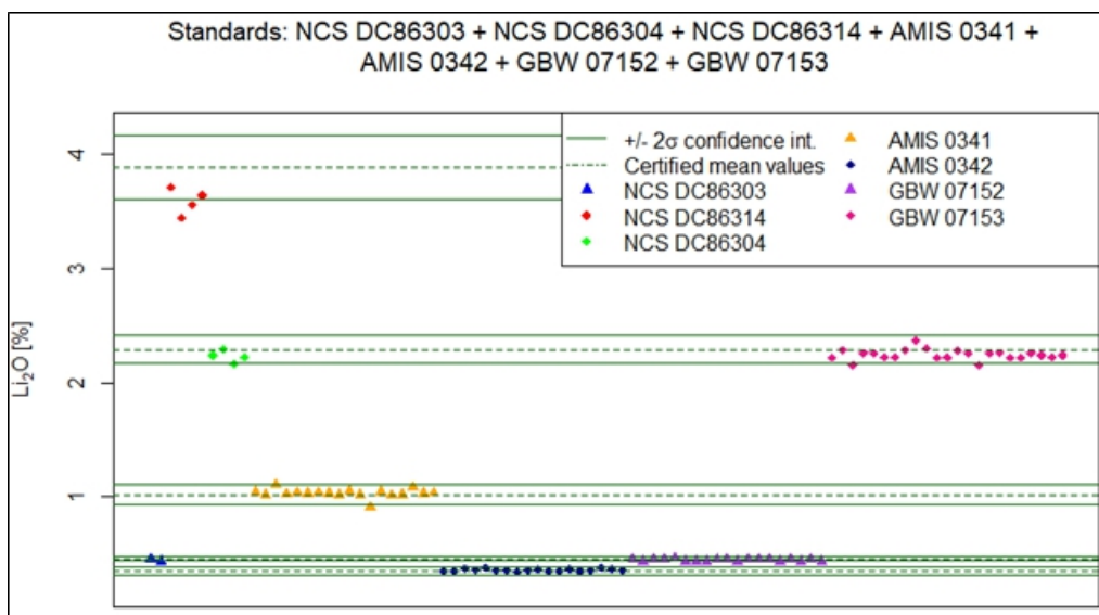
Figure 8-2: Control chart showing the performance of the various reference materials used for the 2016–2021 programs
