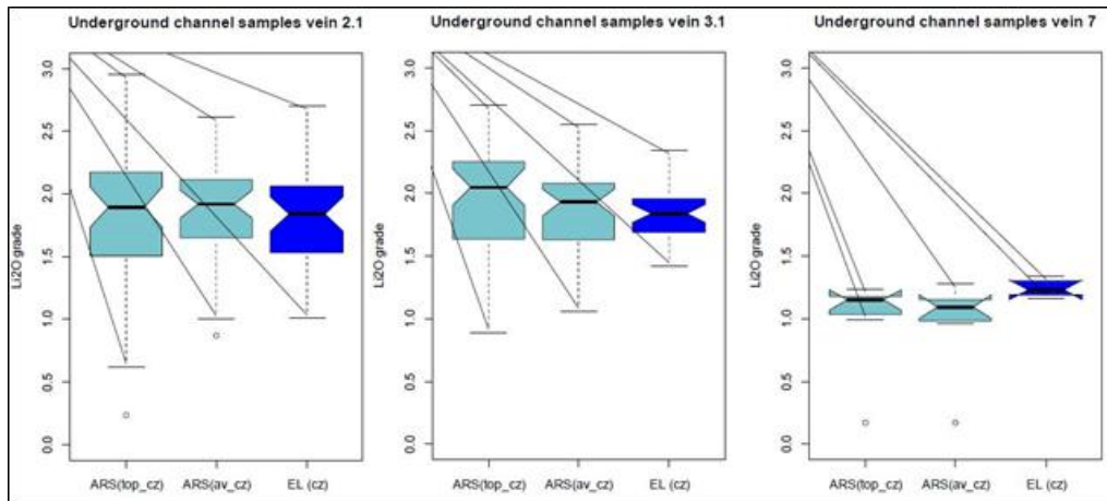
Figure 9-2: Summary of the comparison and verification investigation for all three veins (light blue is the historical data; dark blue are the results of the work completed by European Lithium)
