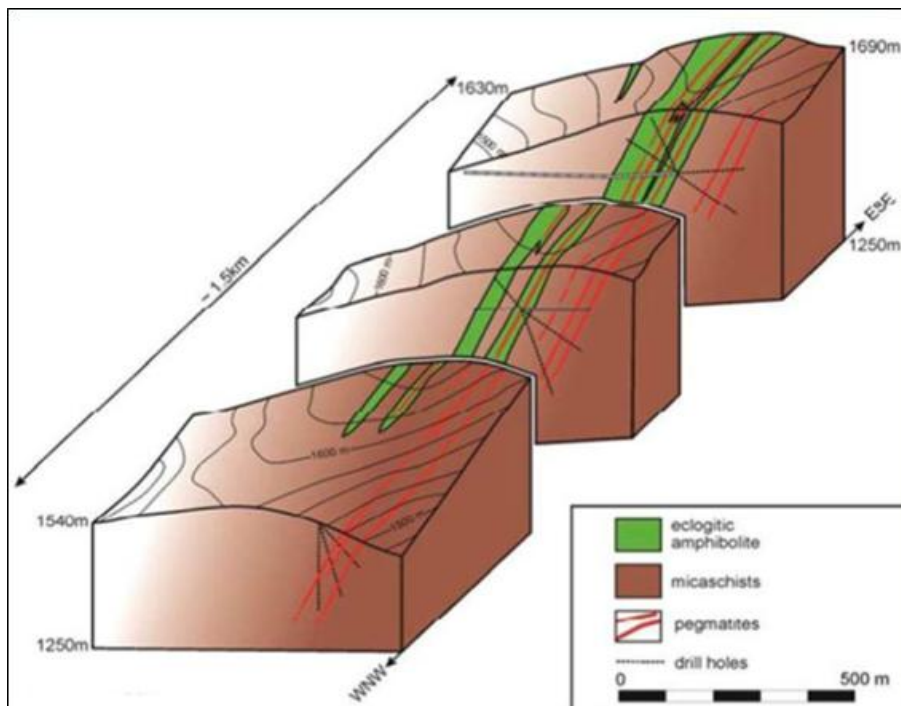
Figure 6-8: 3D schematic of the Wolfsberg pegmatites
