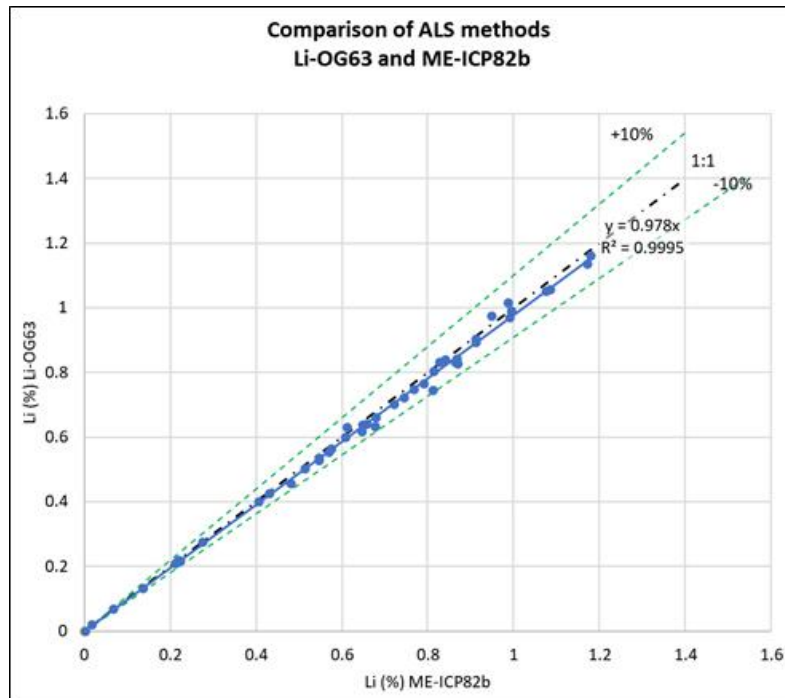
Figure 8-6: Results of 44 samples analysed by Li-OG63 (four-acid digest) and ME-ICP82b (peroxide fusion) at ALS in 2017
