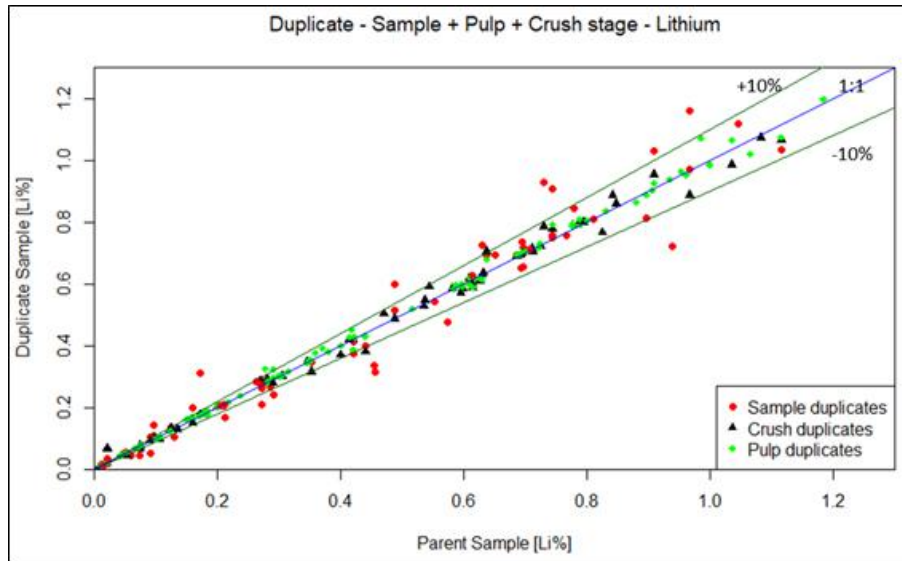
Figure 8-4: Plot of original (parent) vs duplicate sample (core, crush and pulp duplicates) for the 2016–2021 drilling
