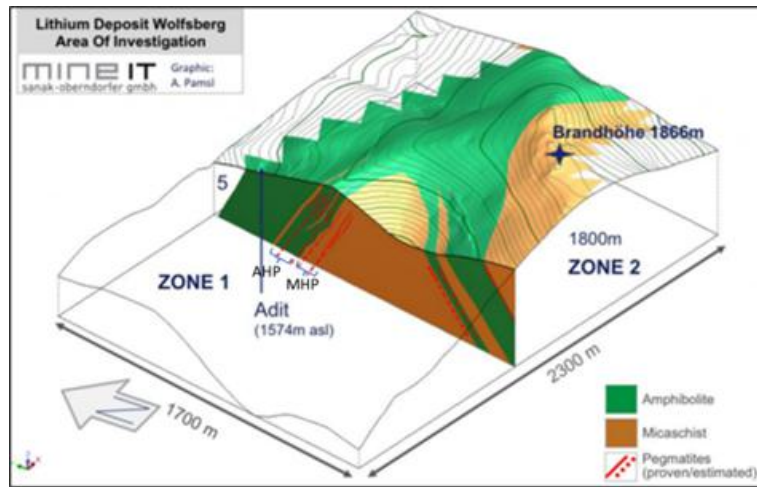
Figure 6-6: 3D representation of anticline showing the relationship between Zone 1 and 2 and the AHP and MHP (see Figure 6-5 for location of section line)
