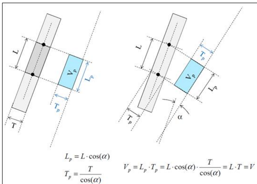
Figure 11-3: Relationship between volume in 3D and 2D showing the impact of the projection plane
